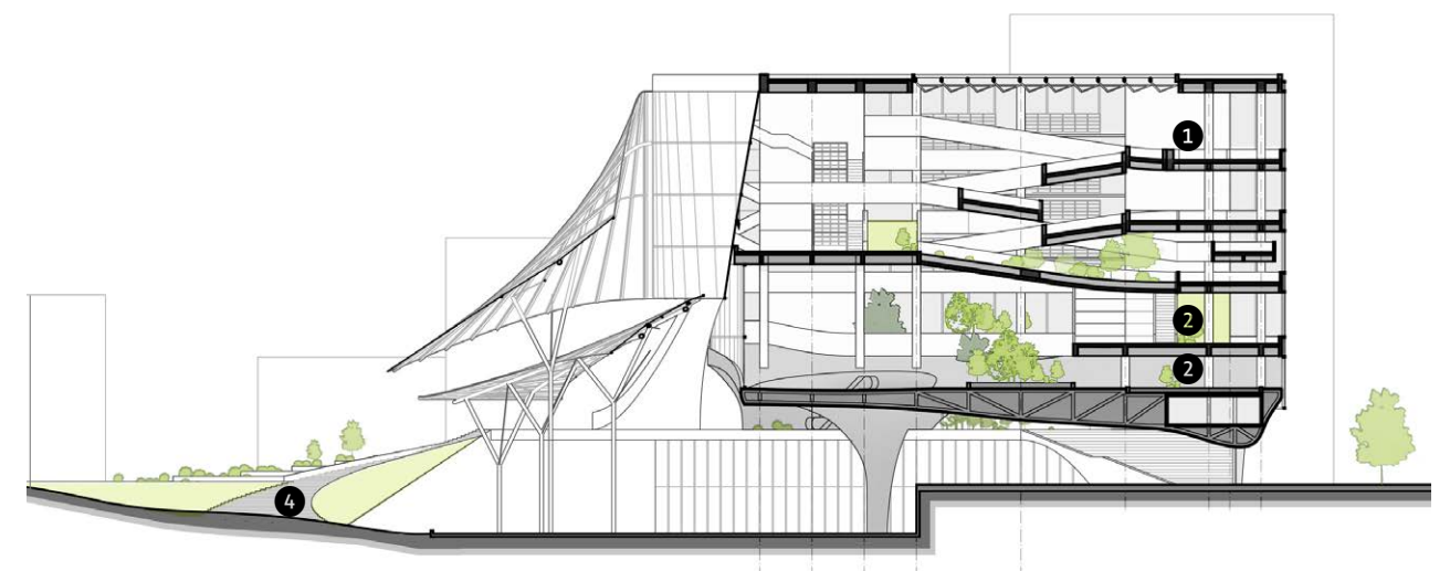
Section B-B 1:800
